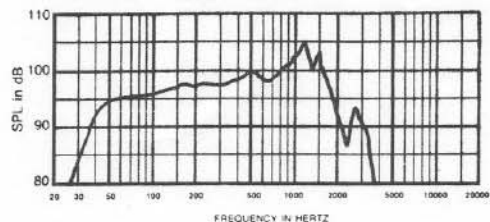
FIGURE 1 — Axial Frequency Response, 1 Watt/1 Meter, 10-Cubic-Foot Enclosure
