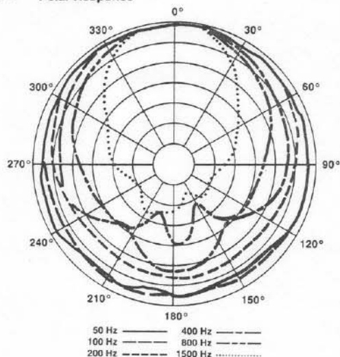
FIGURE 6 — Polar Response
